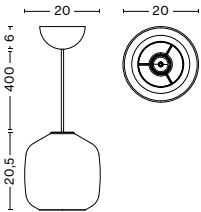
ASPEKT BUOY GLASS PENDANT 200 Diameter 20 cm Height 20,5 cm Weight 1,7 kg
