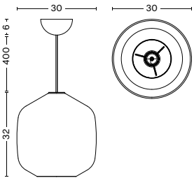
ASPEKT BUOY GLASS PENDANT 300 Diameter 30 cm Height 32 cm Weight 3,3 kg
