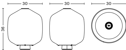
ASPEKT BUOY GLASS TABLE LAMP 300 Diameter 30 cm Height 36 cm Weight 4,5 kg
